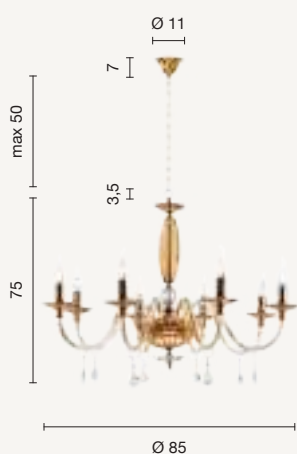
lampadario chandelier LP.CECILIA/8-ORO LP.CECILIA/8A LP.CECILIA/8-TORT power: 8 x E14 voltage: 220-230V
