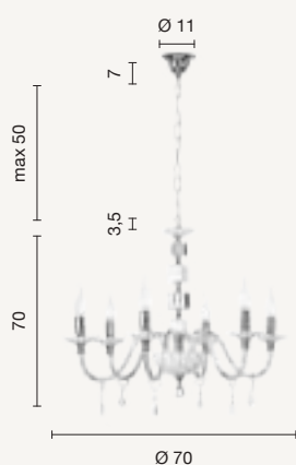
lampadario chandelier LP.LIVIA/6BL LP.LIVIA/6-TOR LP.LIVIA/6-FUME LP.LIVIA/6-OTT power: 6 x E14 voltage: 220-230V
